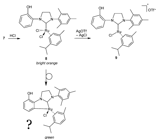
Scheme 3. Losing the chelate effect.
