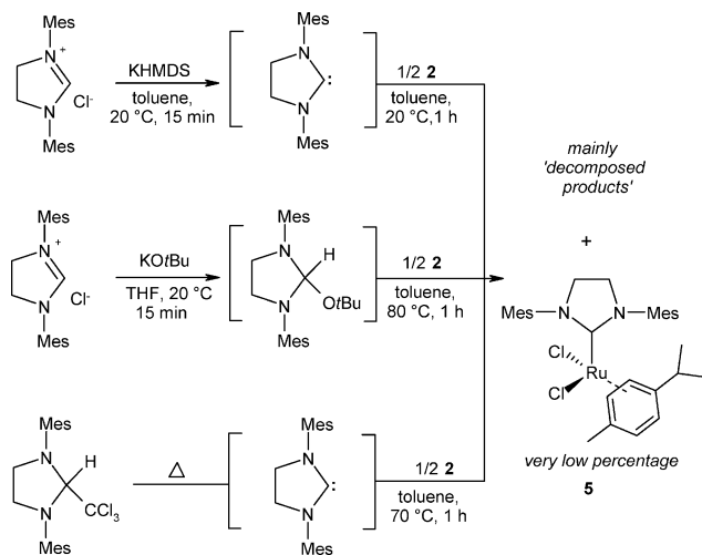
Scheme 1. Synthesis of [( p -cymene)(H 2 IMes)RuCl 2 ].
