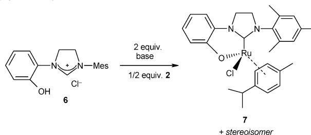
Scheme 2. Synthesis of NHC-arene complex 7 .
