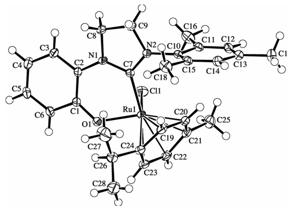
Figure 1. The molecular structure of 7 ; ellipsoids show 50% probability.
